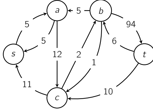
Figure 2: The residual network given the flow presented in Fig. 1.
